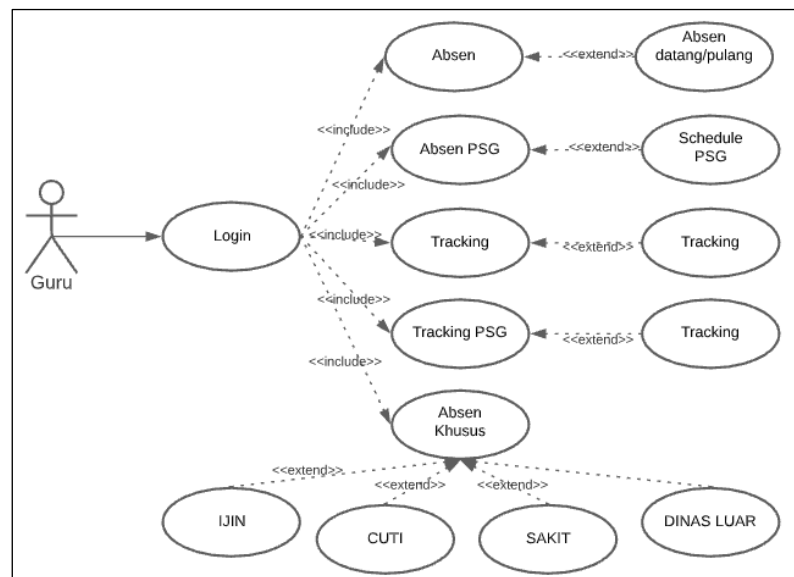
Gambar 2. Use Case Diagram Guru
