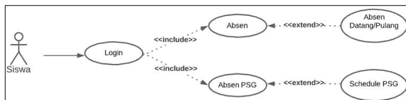
Gambar 3. Use Case Diagram Siswa
