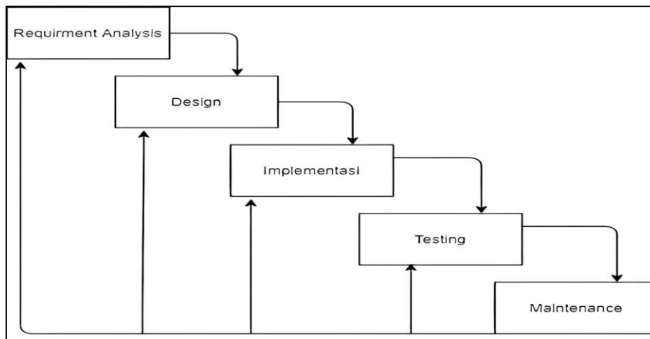
Gambar 1. Metode Waterfall
