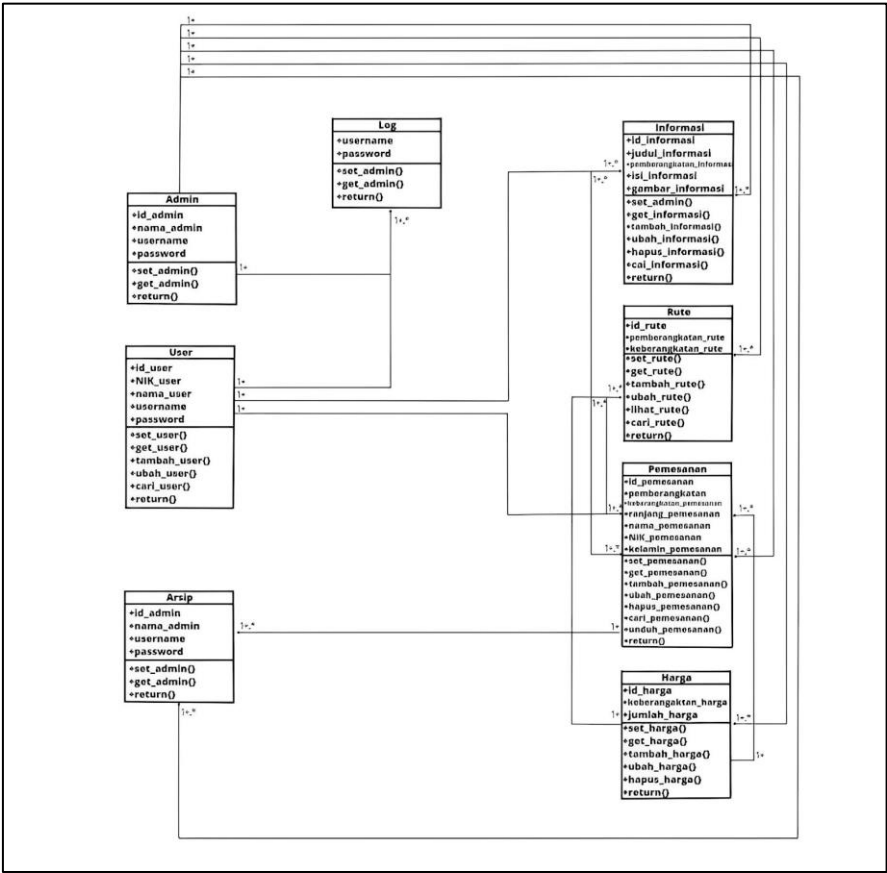
Gambar 3. Class Diagram
