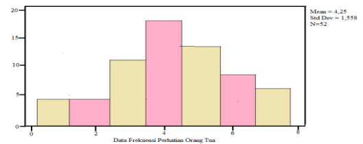
Gambar 2.1 Histogram Perhatian Orang Tua
