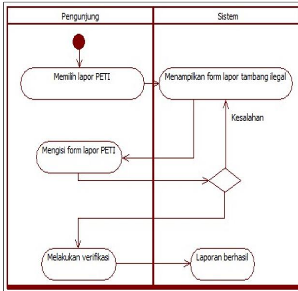
(a) Activity Diagram Lapor PETI
