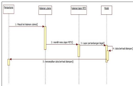
(a) Sequence diagram Lapor PETI Pertambangan
