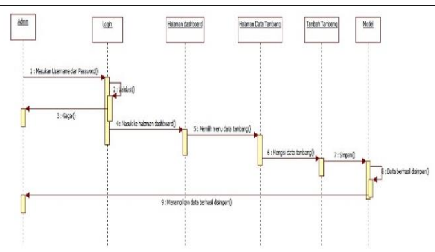
(b) Sequence diagram Lapor PETI tambah Data
