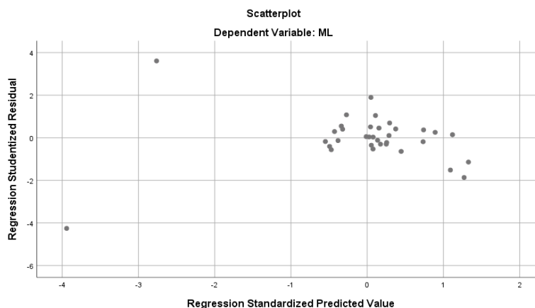
Gambar 2. Scatterplot
